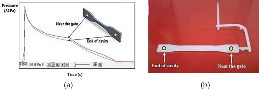
Figure 1: (a) Image for the location of pressure sensors with cavity pressure profile and (b) moulded dumbbell with feed system
