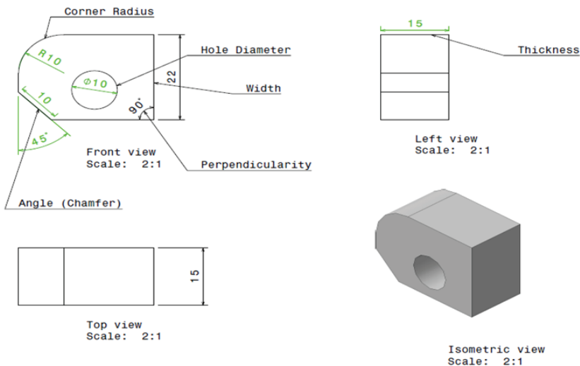
Figure 4: Geometry of the test specimen
