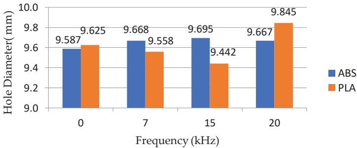
Figure 7: Graph for hole diameter vs frequency of ABS and PLA
