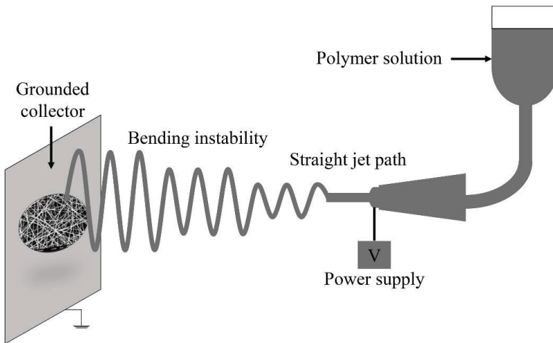
Figure 1: Schematic diagram of electrospinning process
