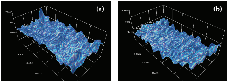
Figure 4: 3D view of surface texture: (a) 120-grit size (b) 150-grit size
