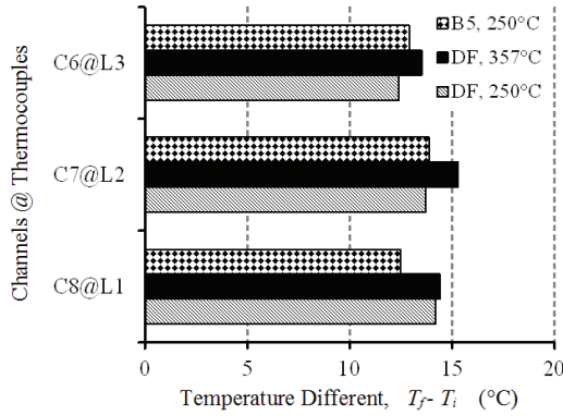
Figure 6: Temperature difference measured by left side thermocouples
