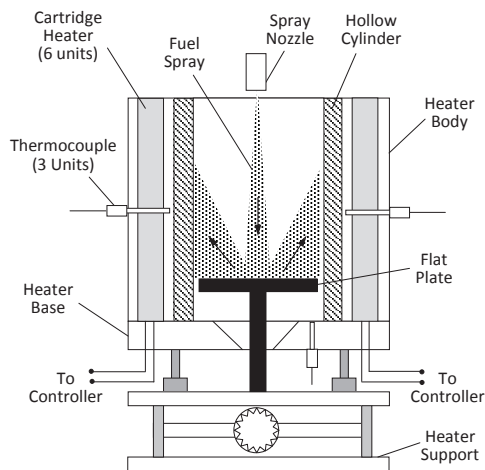
Figure 1: A hollow cylinder heater apparatus
