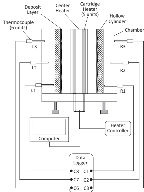
Figure 2: Heat transfer chamber apparatus
