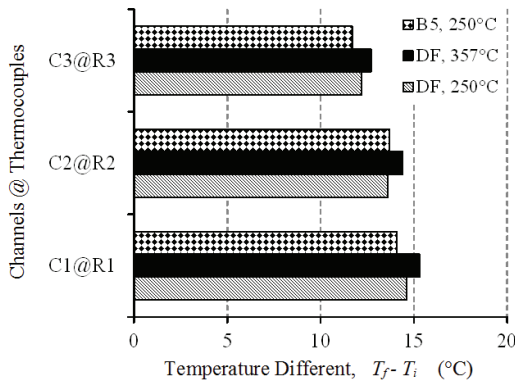
Figure 7: Temperature difference measured by right side thermocouples
