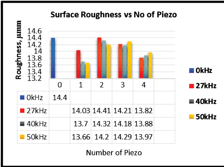
Figure 6: Graph surface roughness versus number of Piezo
