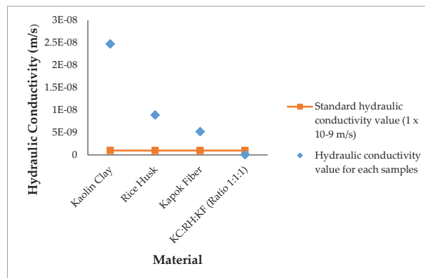
Figure 6: Hydraulic conductivity value for each material in comparison with standard [8]
