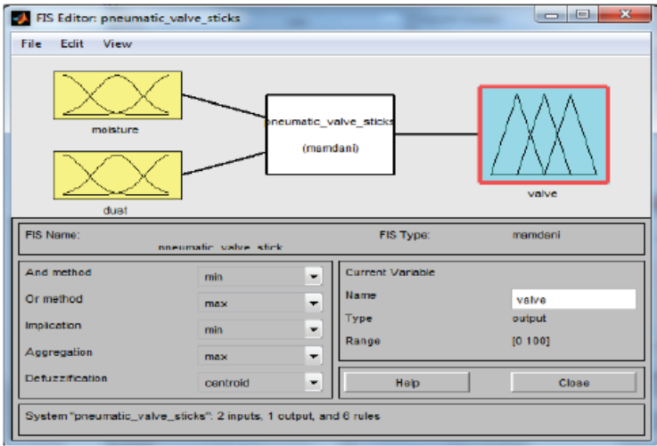
Fig 5.1: Fuzzy Inference System (FIS) Editor
