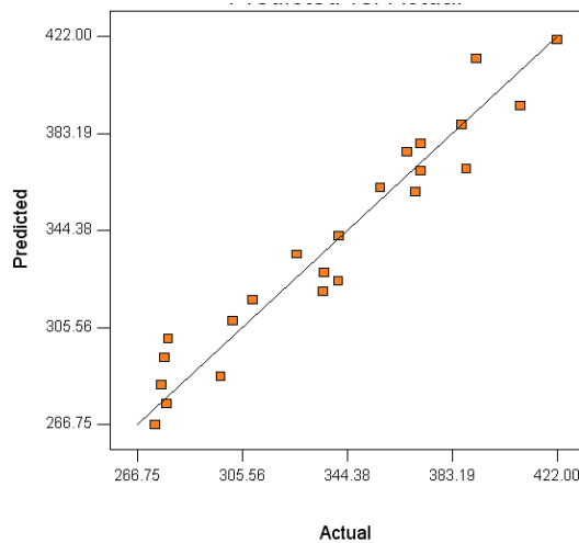
Figure 6: Prediction vs actual value of subsurface microhardness
